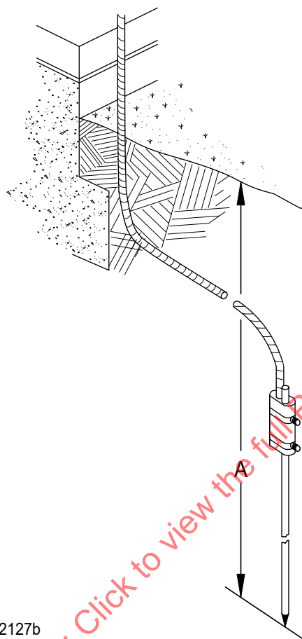
Figure 10.1 Grounding in Moist Clay Type Soil
