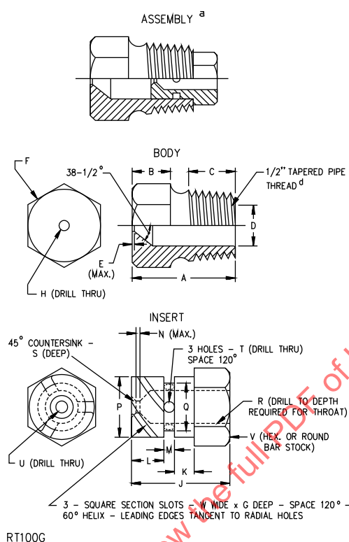
Figure 84.1 Rain-test spray head
