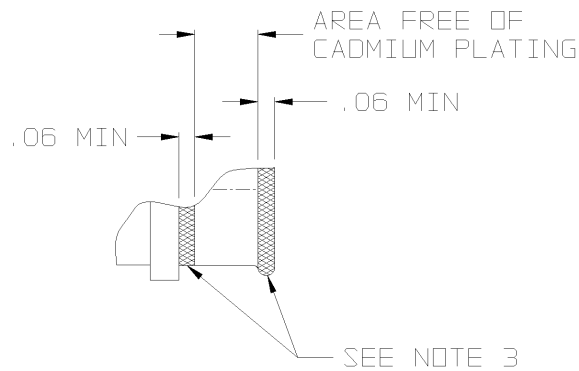
FIGURE 2 - SELECTIVE PLATING
