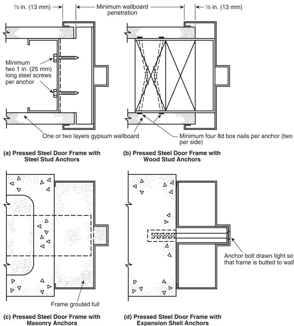
FIGURE A.6.3.1.2 Typical Pressed Steel Door Frame Installations.
