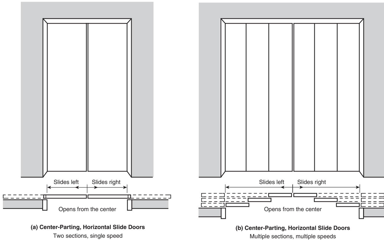
FIGURE A.14.2.3(b) Center-Parting, Two-Section, Single-Speed Doors and Multiple-Section, Multiple-Speed Horizontally Sliding Doors. (Courtesy of ASME A17.1/CSA B44-2010, Safety Code for Existing Elevators and Escalators .)
