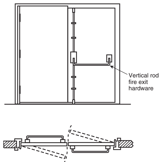
FIGURE A.3.3.41 Double Egress Door and Frame.
