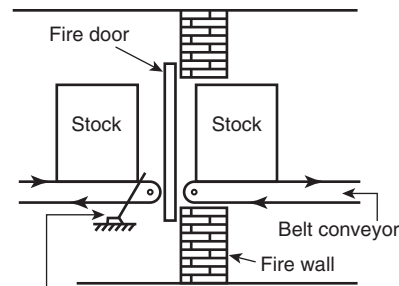
FIGURE B.4(a) Protection of Opening Where Belt Conveyor Can Be Interrupted.
