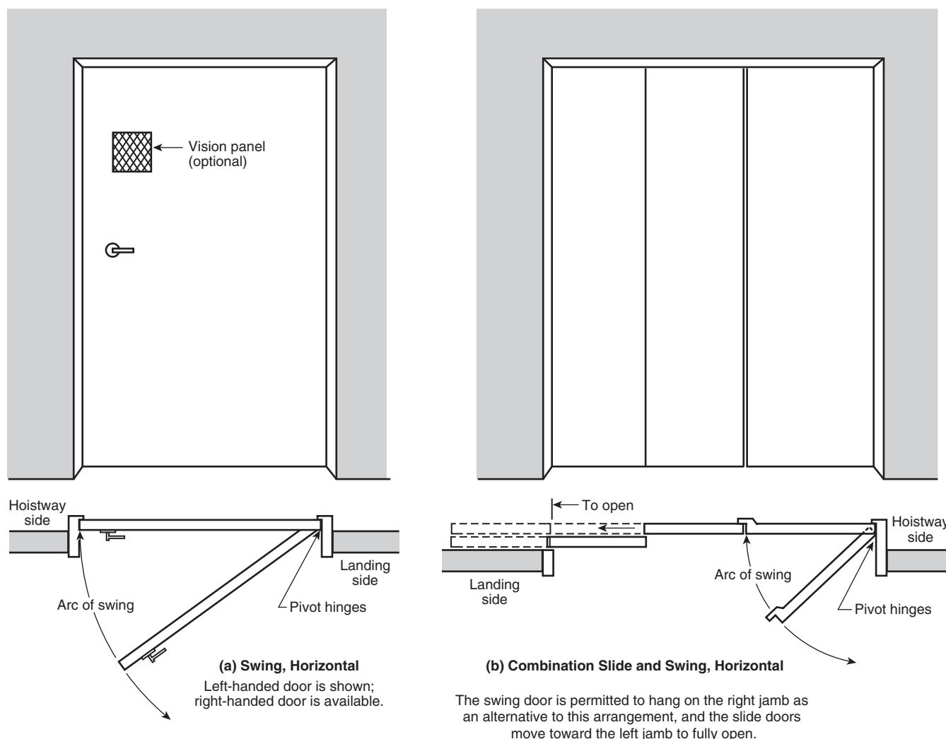
FIGURE A.14.2.1.3 Horizontal Swinging and Horizontal Combination Sliding and Swinging Doors. (Courtesy of ASME A17.1/CSA B44-2010, Safety Code for Existing Elevators and Escalators .)
