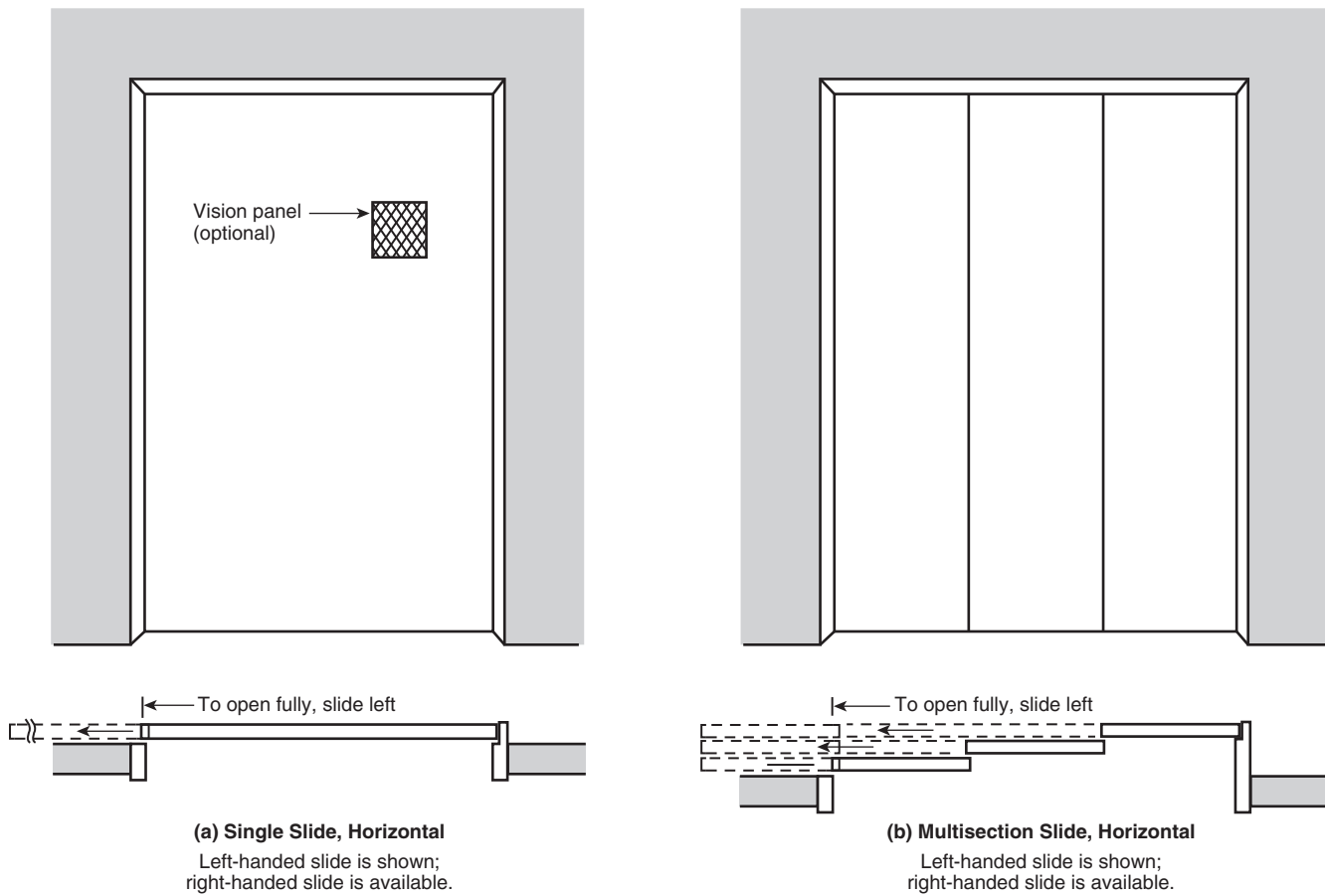
FIGURE A.14.2.2.3(a) Horizontal Single Sliding and Horizontal Multisection Sliding Doors. (Courtesy of ASME A17.1/CSA B44-2010, Safety Code for Existing Elevators and Escalators .)
