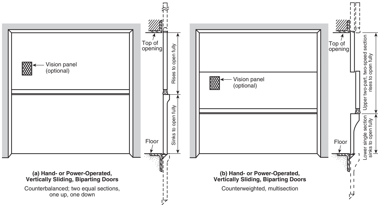
FIGURE A.14.2.3(b) Hand- or Power-Operated, Vertically Sliding, Biparting and Slide-Parting Doors. (Courtesy of ASME A17.1/CSA B44-2010, Safety Code for Existing Elevators and Escalators .)
