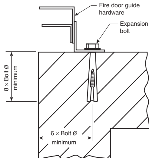
FIGURE A.4.8.6(a) Corner Walls.
