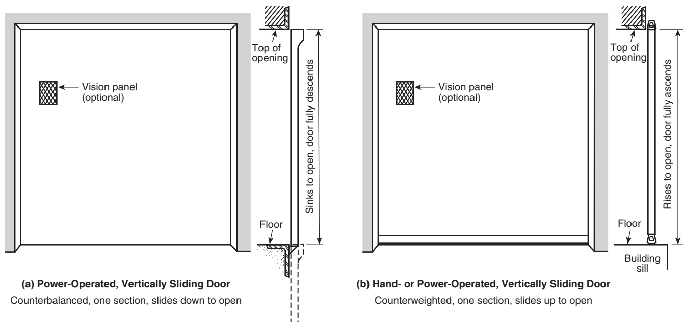
FIGURE A.14.2.3(a) Power-Operated, Vertically Sliding Door and Hand- or Power-Operated, Vertically Sliding Door. (Courtesy of ASME A17.1/CSA B44-2010, Safety Code for Existing Elevators and Escalators .)
