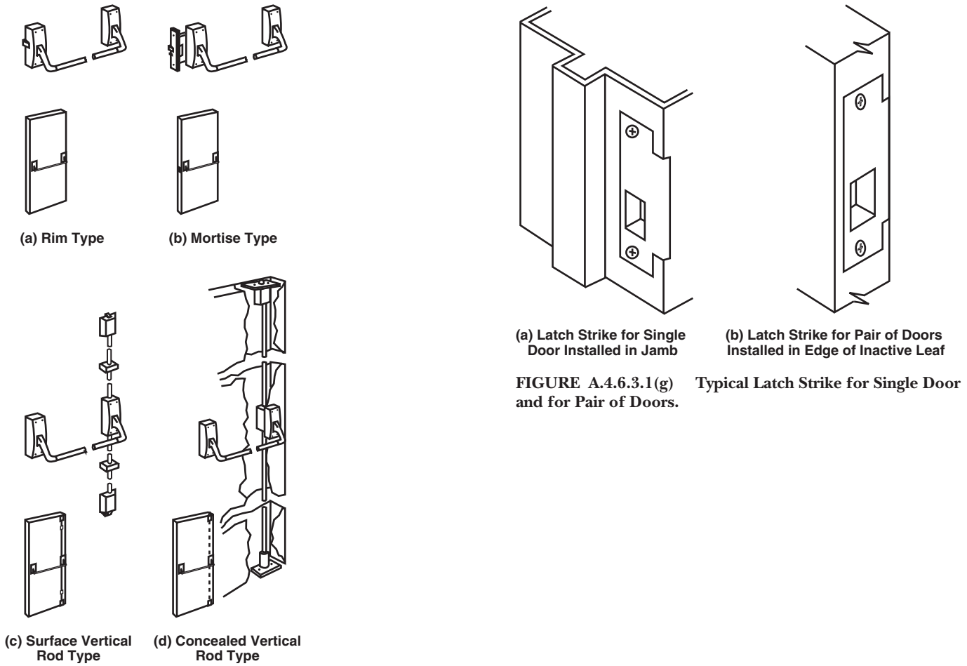
FIGURE A.4.6.3.1(e) Types of Fire Exit Hardware.
