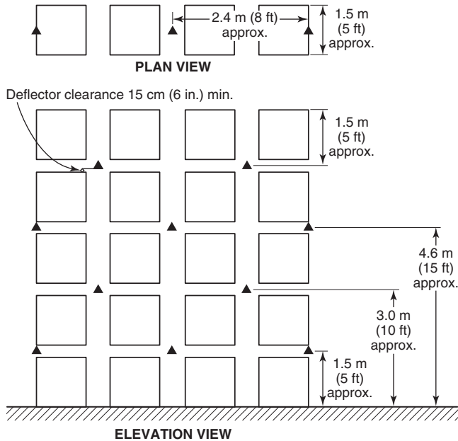
(1) Single Row Racks
