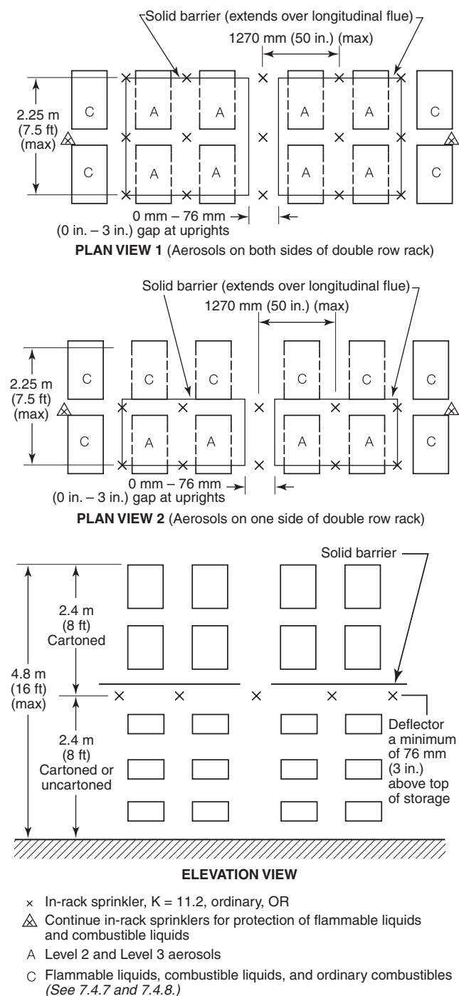
FIGURE 7.4.1 Special Protection for Level 2 and Level 3 Aerosol Products in Double-Row Racks.
