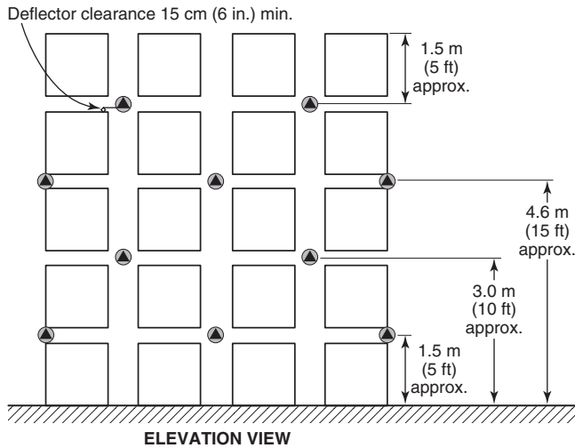
(2) Double Row Racks
