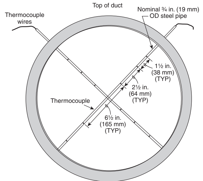
FIGURE 5.1.1 Flue Thermocouple Layout.
