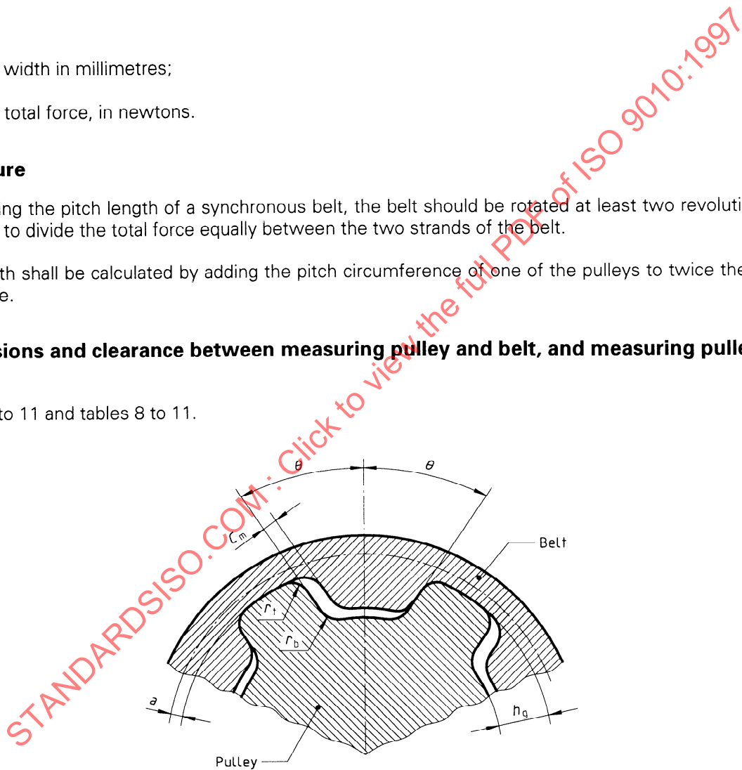
Figure 6 — Dimensions and clearance between measuring pulley and belt for types ZA and ZB (see table 8)
