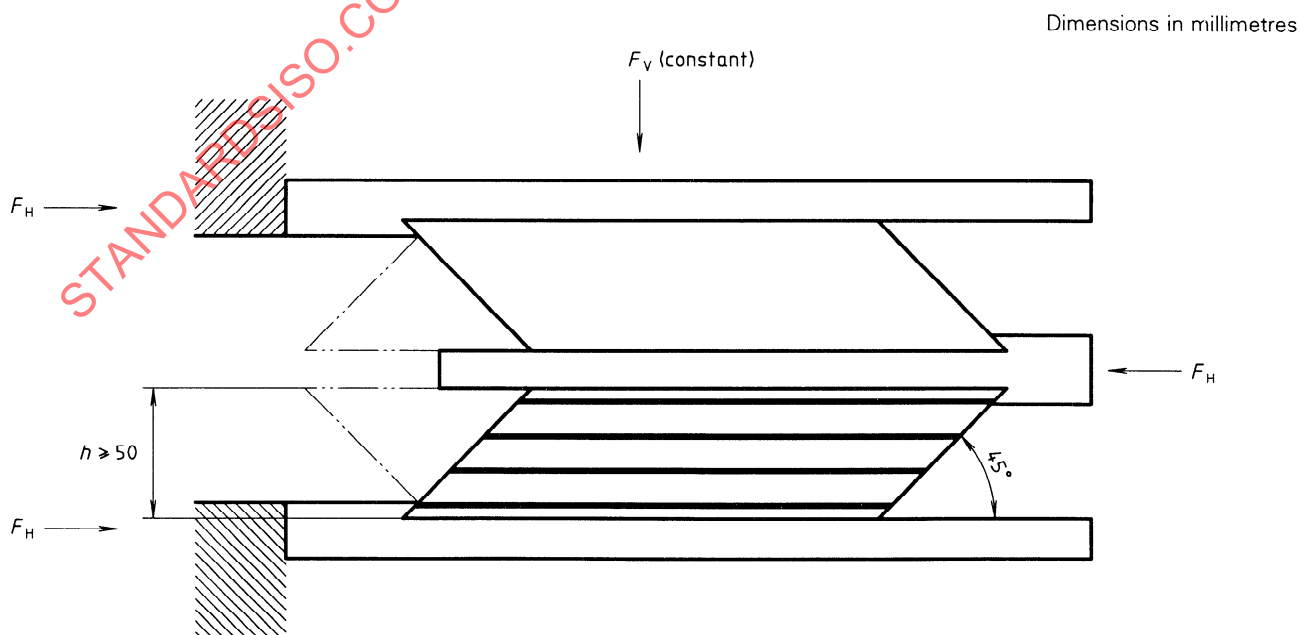
Figure A.1 — Shear-break test piece and test
