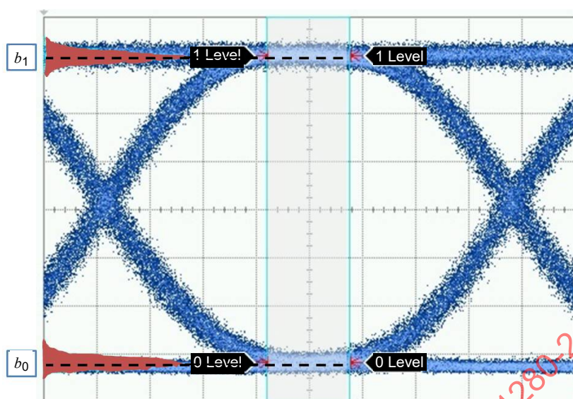
Figure 4 – Histograms centred in the central 20 % of the eye used to determine the mean logic one and 0 levels, b_1 and b_0
