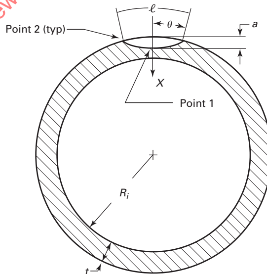
Figure A-3540-1 Cylindrical Semielliptical Outside Surface Flaw Geometry
