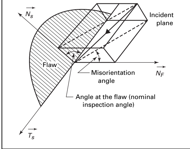
Figure VIII-S5-1 Misorientation Angle
